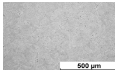
Microstructure after low solution anneal
